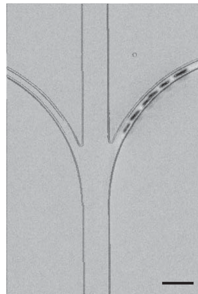
Figure 3 | Quantification of cells displaying a preference to travel to the right by using a microchannel junction. Cells travelling along the right channel wall (closer to the floor of the microchannel) enter the right sidearm; cells travelling along the left channel wall (closer to the ceiling of the microchannel) enter the left sidearm. Six smooth-swimming E. coli (HCB437) cells 27 are shown entering the right sidearm. Scale bar, 20 \mu\text{m} .
