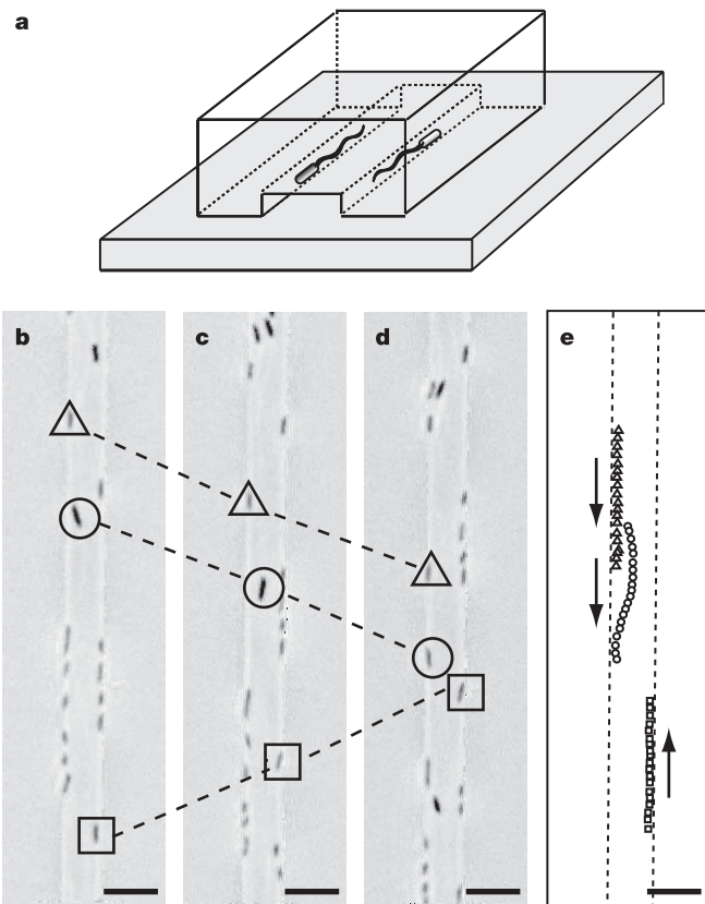
Figure 2 | Images of cells in composite agar/ox-PDMS microchannels. a , An oxidized PDMS film with embossed channels seals conformally to an agar substrate and forms liquid-filled channels into which E. coli swarmer cells migrate. Within these microchannels (imaged from above), cells that are closer to the floor of the channel swim clockwise or move to the right. b–d , Three time-lapse images showing E. coli swarmer (AW405) cells 26 moving on the right in confining, rectangular microchannels (1.4 \mu\text{m} tall and 7 \mu\text{m} wide) in which nutrient agar formed the floor of the channel and an ox-PDMS film formed the walls and ceiling of the channel. b , t = 0 s; c , t = 0.33 s; d , t = 0.67 s. e , The trajectories of three selected cells between images b and d are shown. Scale bars, 10 \mu\text{m} .
