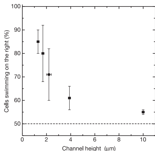
Figure 4 | Preference of cells to move on the right in microchannels as a function of the height of the channel. Channels had a floor composed of nutrient agar, and a ceiling and sidewalls composed of ox-PDMS. For each datum, at least 10 3 cells were counted in seven or more separate channels. Error bars show s.d. for the different channels measured.
