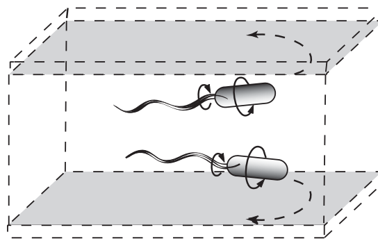
Figure 1 | Cells swim in clockwise, circular trajectories at solid, planar surfaces. When a cell executes a run, all flagella in the bundle rotate anticlockwise (when viewed from behind) and the cell body counter-rotates in a clockwise direction. When viewed from above, the cell trajectories at the bottom surface appear clockwise and the cell trajectories at the top surface appear anticlockwise.
