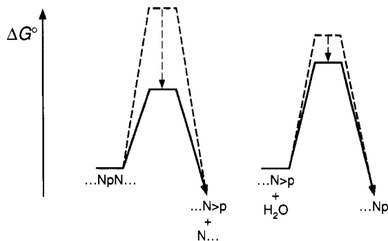
FIGURE 7: Free energy profiles for the reactions in Figure 1. The profiles portray the relative free energy barriers for the ribonuclease-catalyzed (—) or non-enzymatic (- - -) transphosphorylation (left) and hydrolysis (right) reactions. Dashed arrows depict the catalysis effected by ribonucleases.
