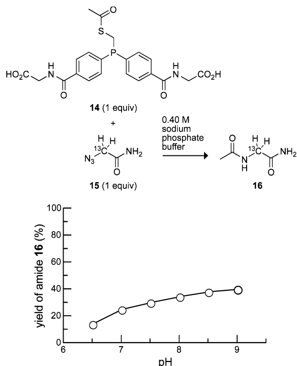
Figure 1. Dependence of the yield of amide 16 on the solution pH in a traceless Staudinger ligation mediated by an acidic phosphinothiothiol. Reactions were performed with equimolar amounts of 14 and 15 (0.16 M) in 0.40 M sodium phosphate buffers of varying pH. ^{13}\text{C} -labeled glycylamide ( ^{13}\text{C} -GlyNH _2 ) is the major product of this reaction at each pH. Data are the mean values (SE = \pm 2\% ) from two or three experiments.
