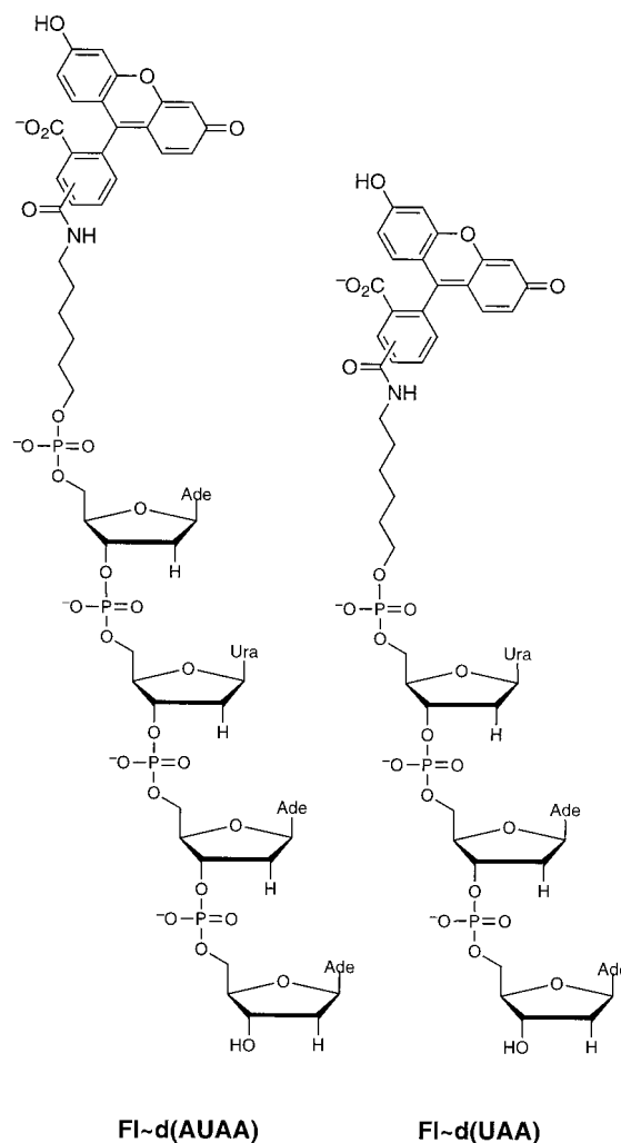
SCHEME 1
