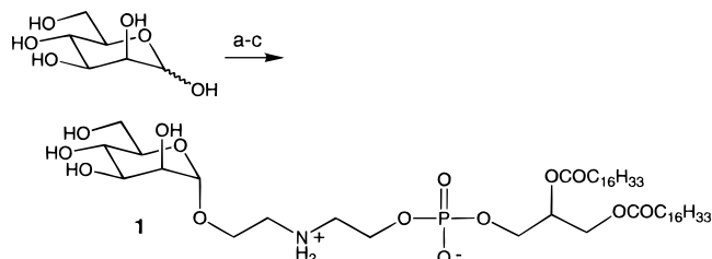
Figure 2. Scheme for synthesis of the glycolipid ( 1 ). (a) Allyl alcohol, Dowex-H + (39% \alpha ). (b) (i) O 3 , 50:50 MeOH/CH 2 Cl 2 ; (ii) PPh 3 . (c) NaCNBH 3 , PEt 3 N, 50:50 MeOH/CHCl 3 (53%, 2 steps).
